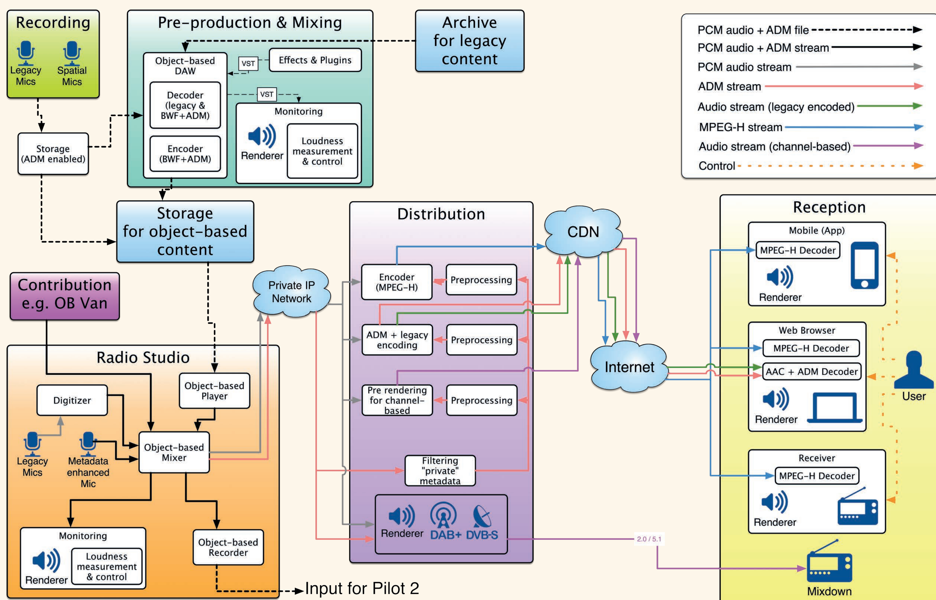
ORPHEUS architecture for object-based production and delivery of audio content (Source: IRT GmbH)
